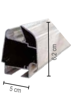
Terminale Like 70
