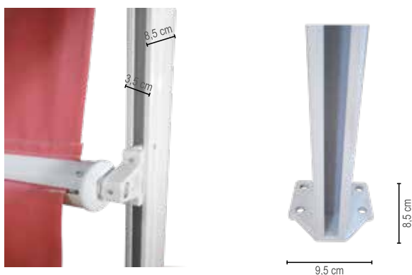
Guida Top Max - Top Max In
