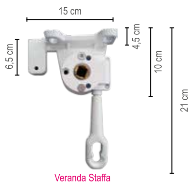
Veranda Staffa
