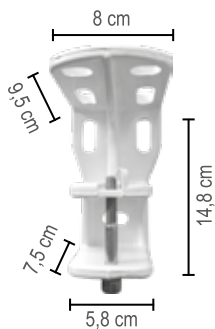
Mensola P/S Like 70
