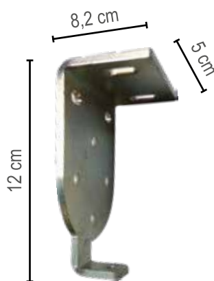
Staffa Energy
