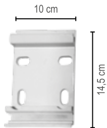
Staffa Newbox
